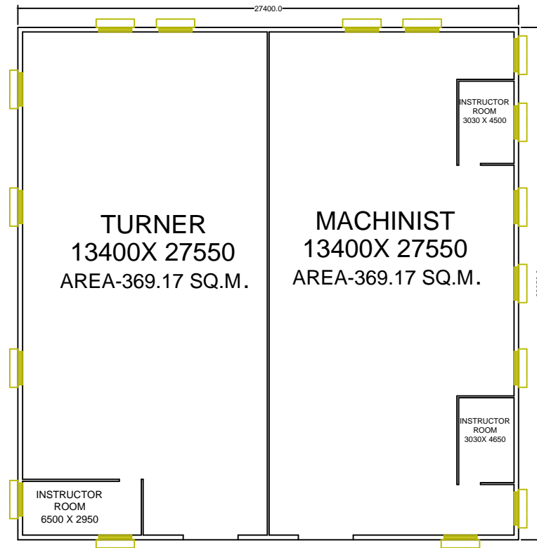
GROUND FLOOR PLAN (SCALE-1:200)
