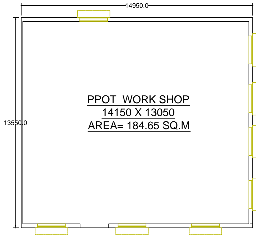
GR FLOOR PLAN (SCALE-1:100)
