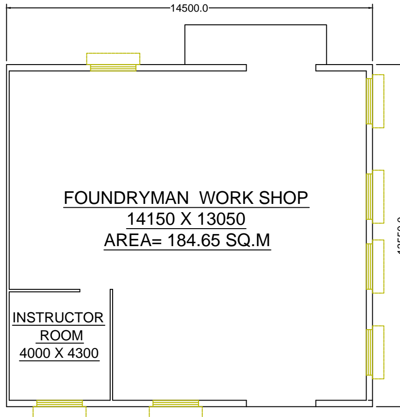
GR FLOOR PLAN (SCALE-1:100)
