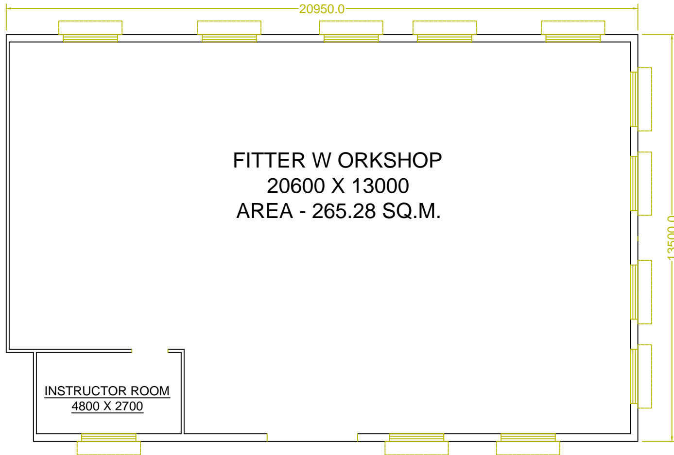
GR FLOOR PLAN (SCALE-1:100)
